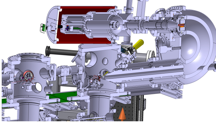
Figure 1.3: Cross-sectional view of the main components of the setup. Preparation chamber (left), measurement chamber (center), energy analyzer (right) and Mott detector (top).
