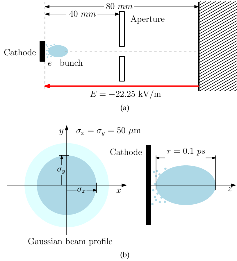
Figure 1.21: (a) Geometry of the simulation. Electrons emitted from a photo cathode are accelerated by a static electric field \vec{E} towards an aperture reproducing the collector entrance to the lens system 40 mm apart. The simulation ends after the remaining electrons have been tracked up to 80 mm away from the cathode. (b) Detail of the electron bunch spatial geometry. Photoelectrons are released from the cathode in a semi-random manner within a time constant on the order of the FEL pulse length. The initial energy and momentum distribution is taken from experimental measurements.
