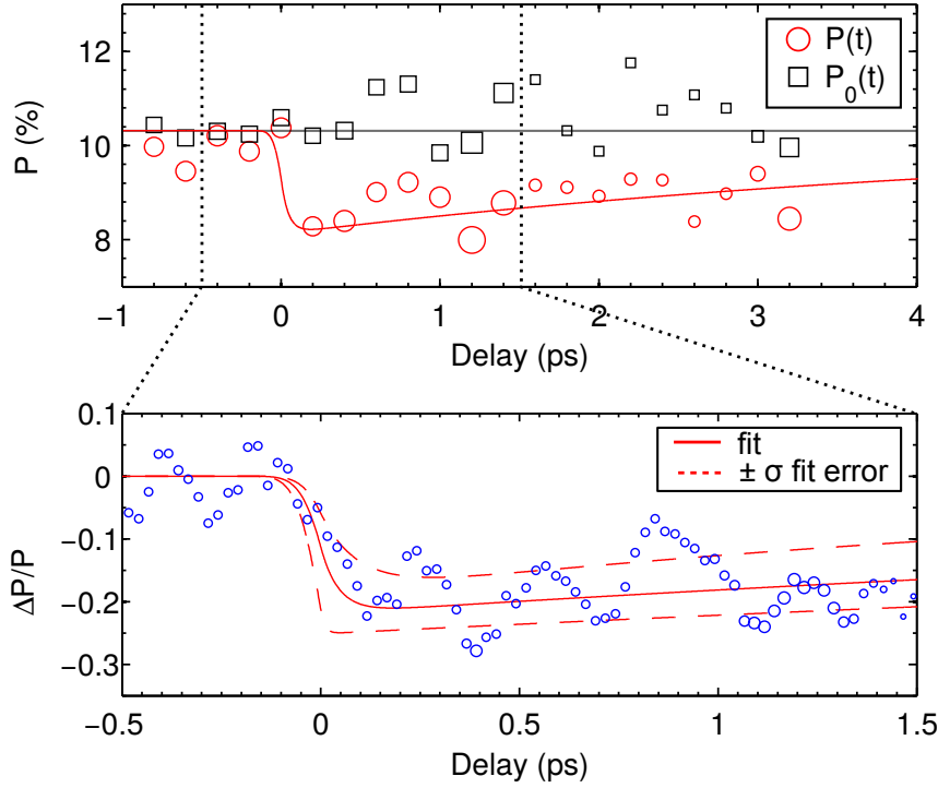
Figure 1.19: Quenching of the magnetization of a 8 ML iron film for two different timescales. In the picture above the polarization of both the pumped P(t) and unpumped P_0(t) signals is depicted. Data bins are 200 fs long. In the picture below the time span has been reduced to allow for a finer time resolution (bin size of 25 fs) and a smoothing filter for signal-to-noise improvement has been applied. The ultrafast magnetization decay on the order of 100 fs (see text description) is clearly visible. The diameter of each point is proportional to the amount of data for that bin. Adapted from [82].
