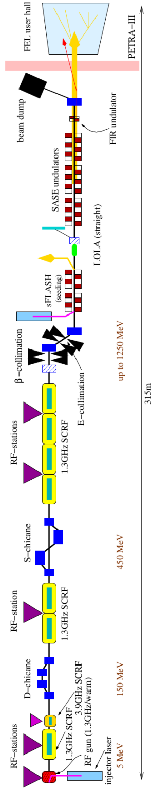
Figure 1.9: Schematics of the FLASH experiment in DESY. Reprinted from [267].
