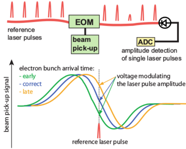
Figure 1.16: Principle of the beam arrival monitor detection. A reference pulse from the train is sampled to the zero crossing of the beam pickup signal inside the EOM. It then undergoes an amplitude modulation when the signal arrives with a certain delay, whose value can be derived from such a modulation. Reprinted from [165].
