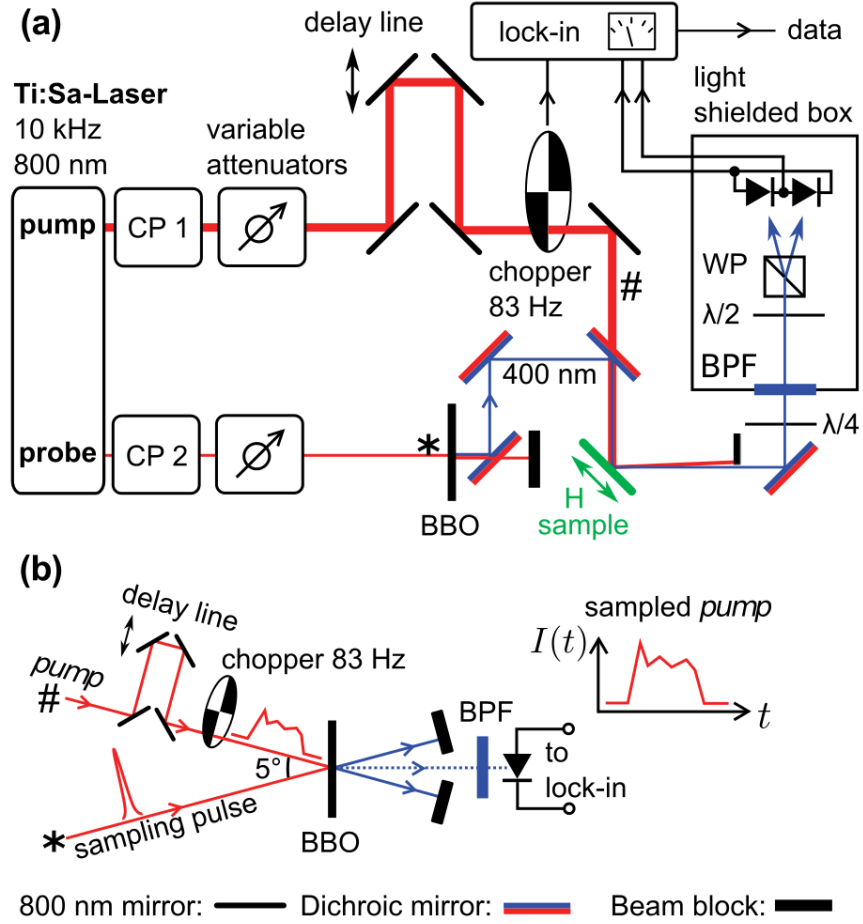
Figure 2.2: (a) MOKE experimental setup for the pulse length variable measurements. The length of the pulses is adjusted through the pump and probe pulse compressors. State-blocking effects are avoided by using a band pass filter with a frequency doubler crystal and a set of dichroic mirrors. (b) Schematic representation of the cross-correlator employed to measure the pulse length, using a 20 fs, 800 nm pulse to sample the pump via up-conversion in a BBO crystal. Reproduced from [83]
