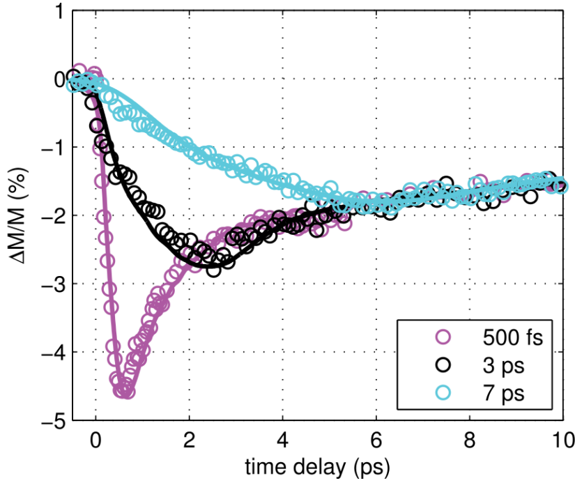
Figure 2.5: Selected experimental demagnetization curves (circles) and the convoluted curves from eq. 2.2 (solid lines) confirm that remagnetization dynamics from picosecond pulses can be reconstructed from femtosecond pulses. Reproduced from [83]
