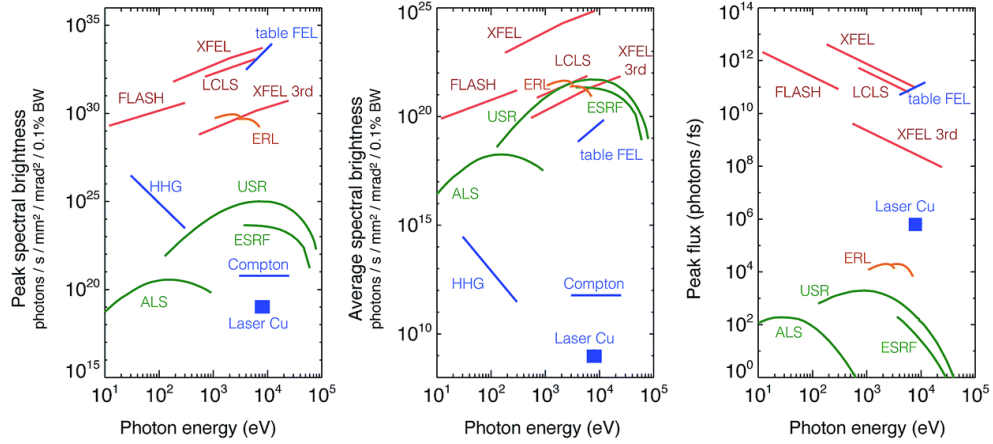
Figure 1.5: Comparison of peak brightness, average brightness and peak peak flux vs photon energy for different x-ray sources. In red the FEL types FLASH (Hamburg, Germany), LCLS (Stanford, USA), XFEL (operational in 2016 in Hamburg, Germany) and ERL (Energy Recovery Linac); in green the synchrotron types USR (Ultimate Storage Ring concept [33]), ALS (Berkeley, USA) and ESRF (Grenoble, France); in blue other sources such as table-top FELs [95], HHG-based sources, Compton scattering or the laser-driven plasma source with Cu target at Max-Born Institut (Berlin, Germany) [287]. Extracted from [49].
